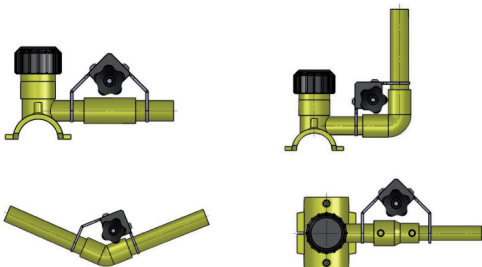
EFRAC Clamp Set for 32mm Diameter
