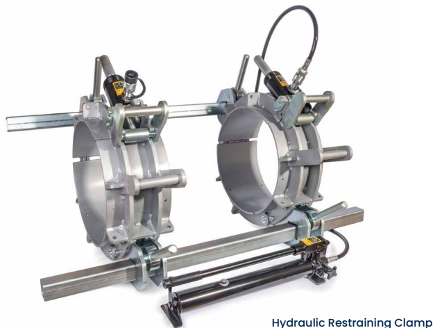
Hydraulic Restraining Clamp
