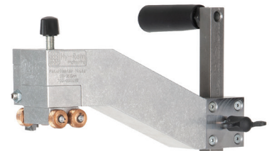
PatchMaster Multi 90-315mm
